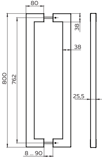
PULL.PH38/800.26 INOX
