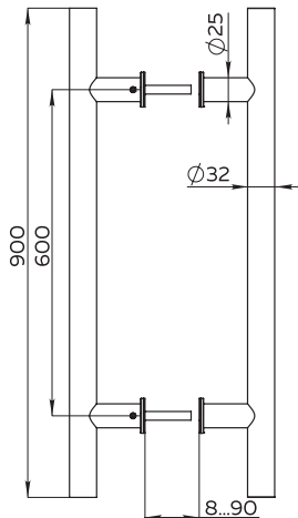
PULL.PH32/900.22 INOX 304 BLACK
