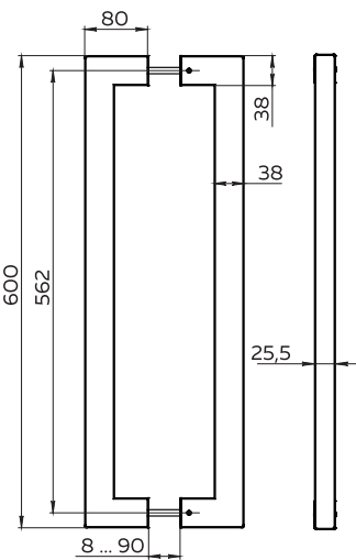
PULL.PH38/600.26 INOX
