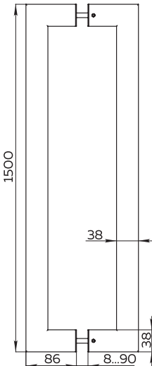
PULL.PH38/1500.26 INOX 304 BLACK
