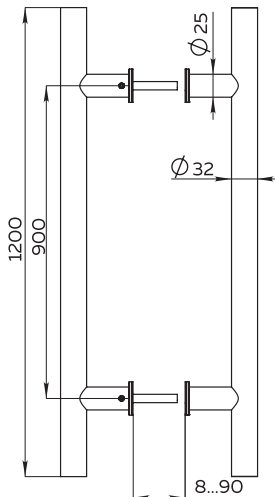
PULL.PH32/1200.22 INOX 304 BLACK
