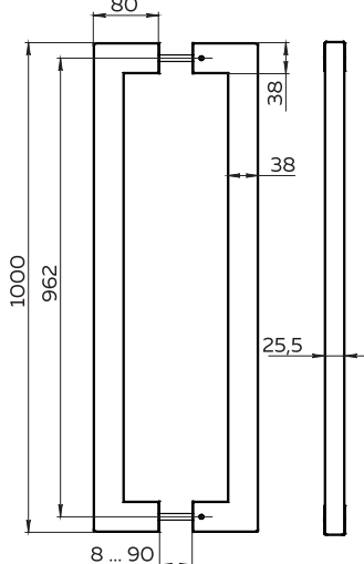
PULL.PH38/1000.26 INOX
